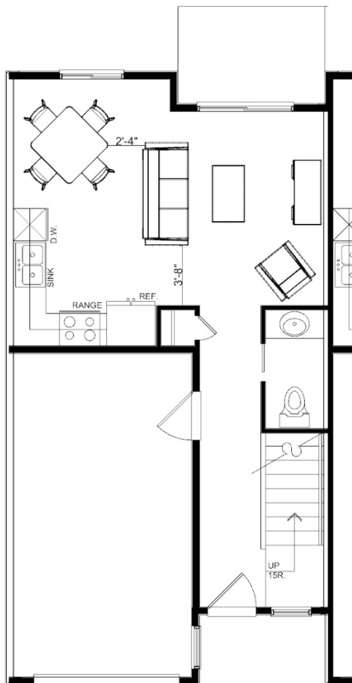
TYPICAL FIRST FLOOR
